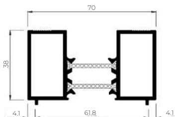
Head extension 38 mm
