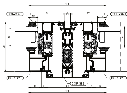
Sash transom sash configuration (standard outer)
