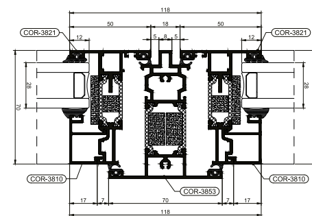
Sash transom sash configuration (flush outer)
