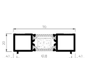
Head extension 20 mm
