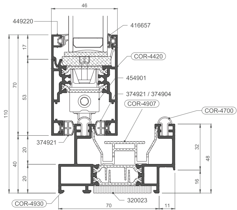
Double-Track Bottom
