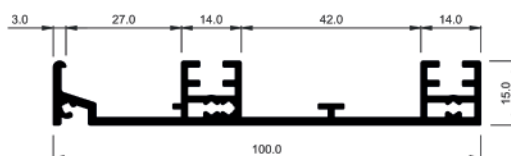
COR-4959 Double-track low threshold (not weather rated - 5-7 week lead time. Anodised silver)
