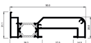
3836 90mm Cill*
