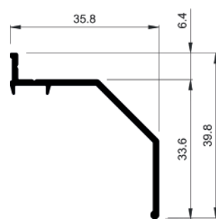
4415 Reduced sash cover
