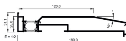
3837 180mm Cill
