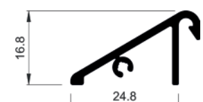
COR-4958 Low threshold ramp (not weather rated - 5-7 week lead time. Anodised silver)
