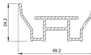
4907 Frame cover
