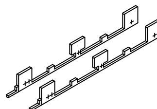
404904 Triple track low threshold end caps
