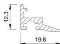
4408 Interlock cover
