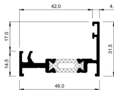
774770 Triple-track 38mm add on
