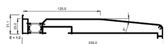
3838 230mm Cill
