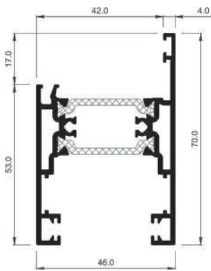
COR-4420 Sash
