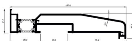
3735 150mm Cill*
