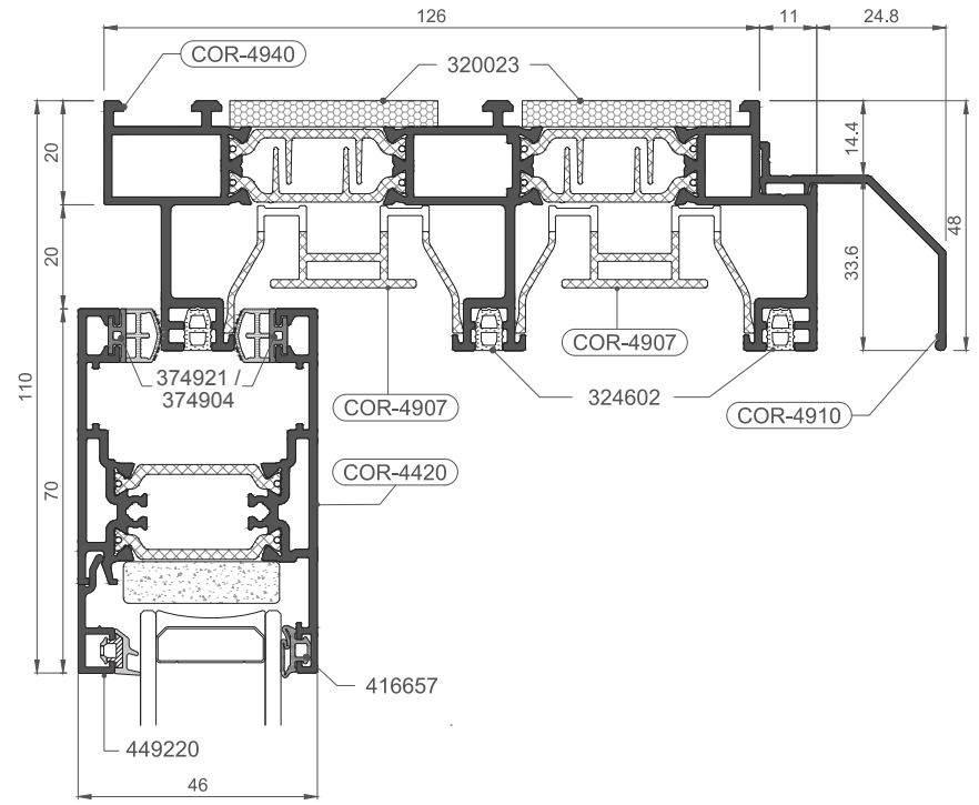
Triple-Track Bottom
