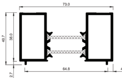
COR-3770 Transom
