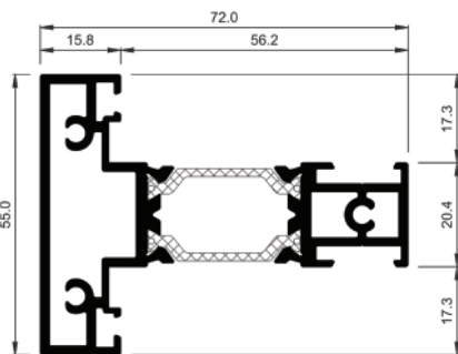
COR-3770 Transom
